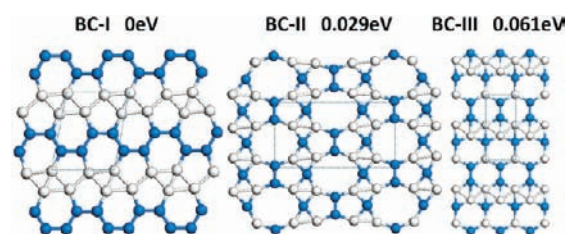
Figure 4. Low-energy 2D structures of BC from the PSO simulations.
