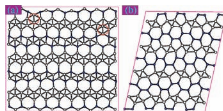
Figure 8. (a) Snapshot of B 3 C-I after a 15 ps MD simulation at 1000 K. The dashed circles denote the newly formed B–B bonds. (b) Snapshot of BC-I after a 15 ps MD simulation at 2000 K.
