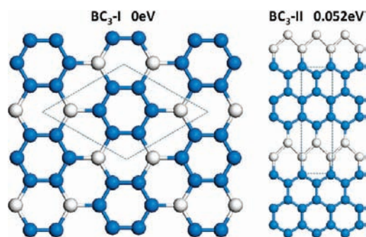
Figure 2. Low-energy 2D structures of BC_3 from the PSO simulations.
