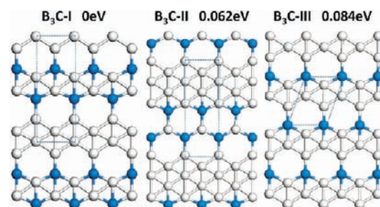
Figure 6. Low-energy 2D structures of B_3C from the PSO simulations.
